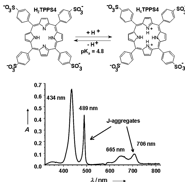
Scheme 1. Top: schematic structure of H_2TPPS4 ( 1 ) and its protonated form ( H^+TPPS4 ). Bottom: absorption spectrum of an aqueous solution of 1 (at pH 3, [NaCl] = 0.3 M). Absorption bands of J-aggregates are at 489 and 706 nm.
