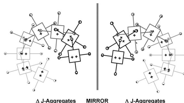
Scheme 2. A possible structure of chiral J-aggregates of 1 .
